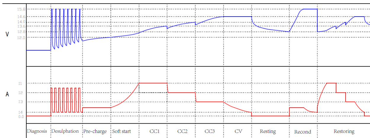
HF(Switch Mode) Charging Steps
